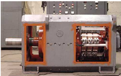
Extensive Testing on Rebuilt Motor
