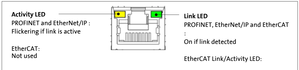
Fig. 3: Fieldbus connector LED
