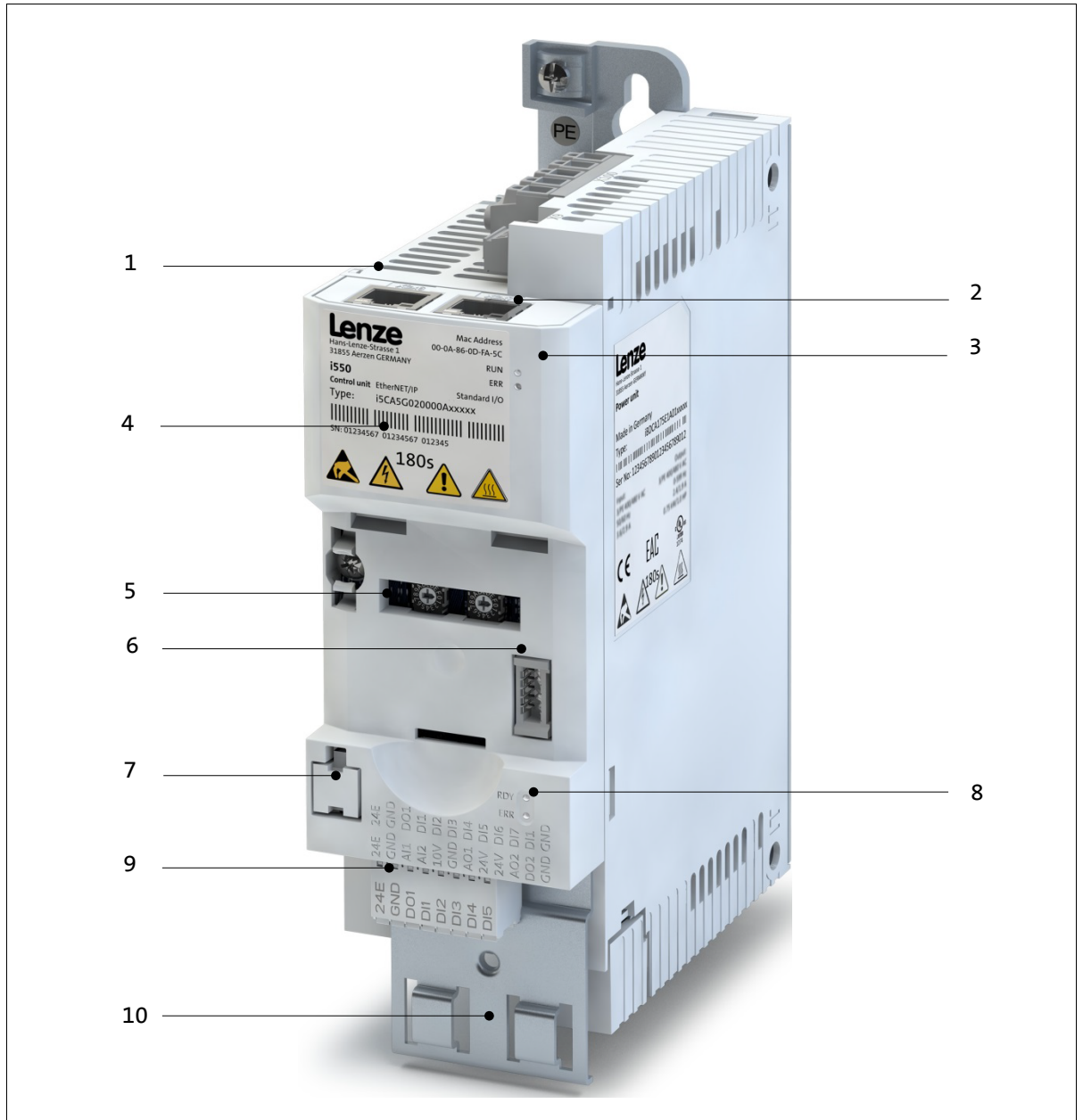
Fig. 1: i550 inverter overview
