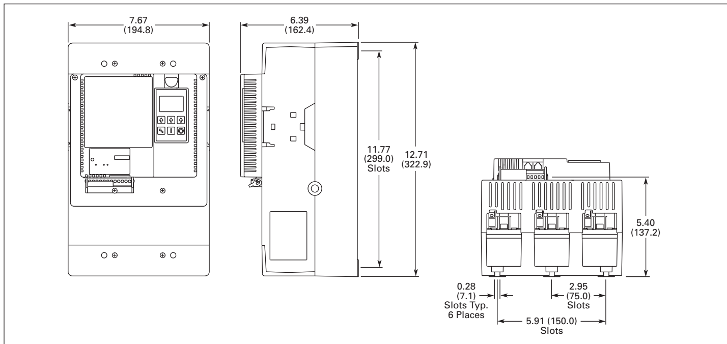
Figure 3. T-Frame (200 mm) S811 Approximate Dimensions in Inches (mm)
