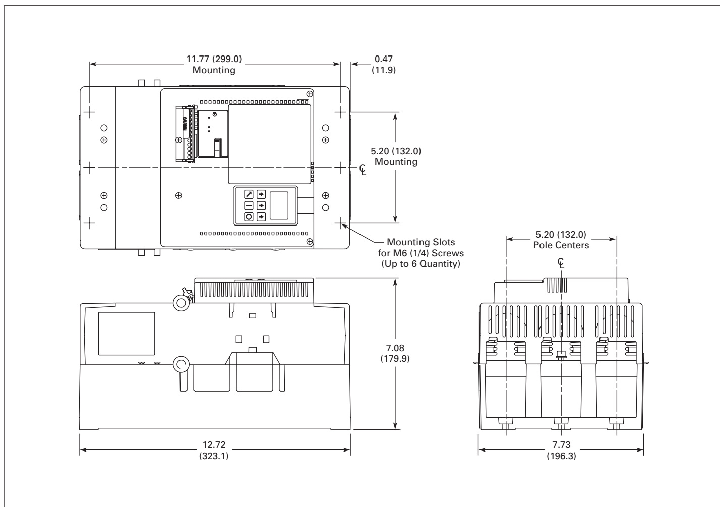
Figure 4. U-Frame (200 mm) S811 Approximate Dimensions in Inches (mm)
