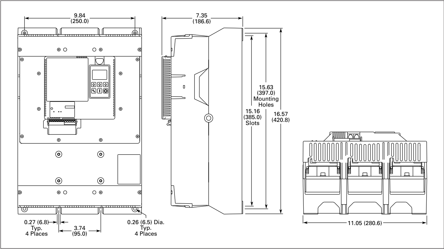
Figure 5. V-Frame (290 mm) S811 Approximate Dimensions in Inches (mm)
